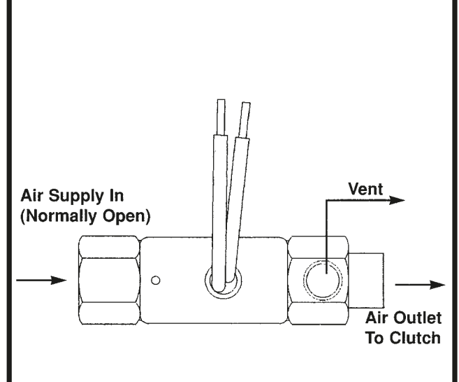
Horton Fan Clutch Control with G.T. Development Corp. Solenoid Valve Part Number 5006-1 (Reference BorgWarner Part Number 1056-08145-01)
