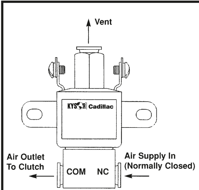
BorgWarner Fan Clutch Solenoid Valve Part Number 1056-07994-01
