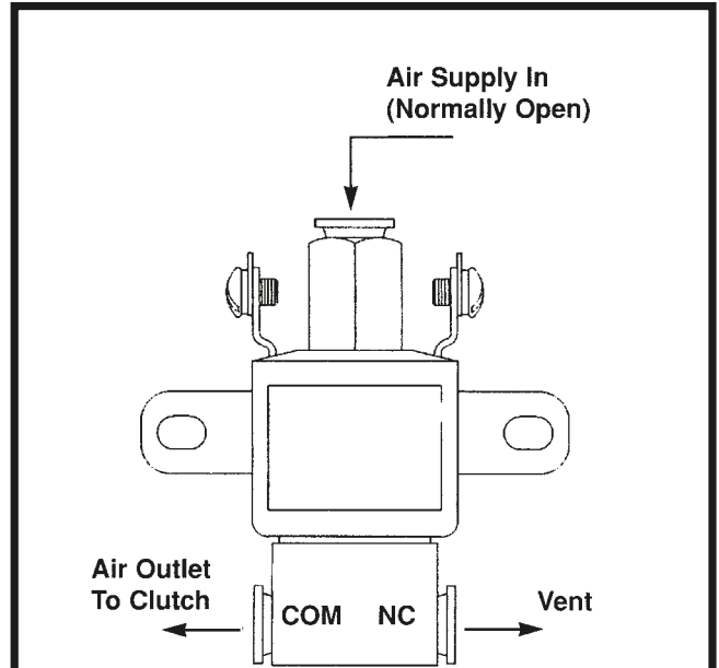
BorgWarner Fan Clutch Solenoid Valve Part Number 1056-07994-01
