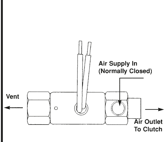
Horton Fan Clutch Control with G.T. Development Corp. Solenoid Valve Part Number 5006-1 (Reference BorgWarner Part Number 1056-08145-01)
